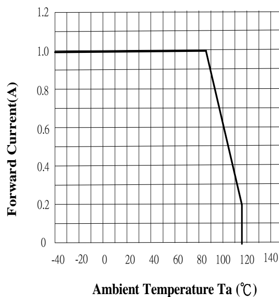
Forward Current & Ambient Temperature
